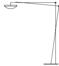
F5 H 2000 mm D 1800 mm Diffuser Ø 400 mm H 120 mm Base Ø 470 mm
