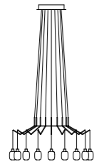
BR9 Ceiling Rose Ø 270 mm Cable 700-1200 mm Diffuser Ø 70 mm H 90 mm
