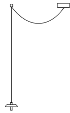
S1L Ceiling Rose Ø 120 mm H 40 mm Lateral Ceiling Attachment Ø 15 mm H 25 mm Cable 3000 mm Diffuser Ø 120 mm H 76 mm
