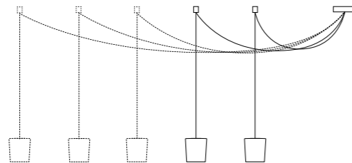
2L - 3L - 4L - 5L Ceiling Rose Ø 180 mm H 40 mm Lateral Ceiling Attachment Ø 15 mm H 25 mm Cable 3000 mm Diffuser Ø 135 mm H 150 mm
